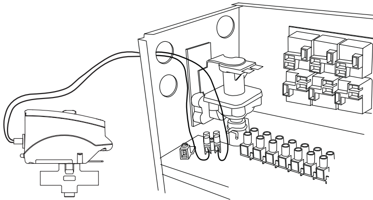
CONNECT DRAIN WIRES THROUGH CONDUIT TO DRAIN TERMINAL BLOCK IN STEAMER:
