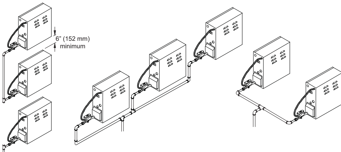
DIAGRAM 4: TYPICAL DRAIN INSTALLATIONS
