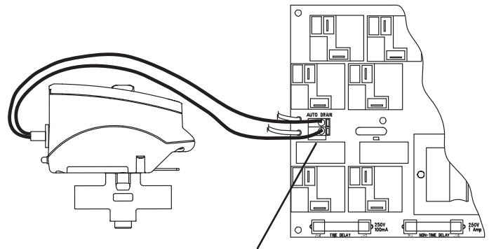
CONNECT DRAIN WIRES THROUGH CONDUIT TO DRAIN TERMINAL BLOCK ON CIRCUIT BOARD:
