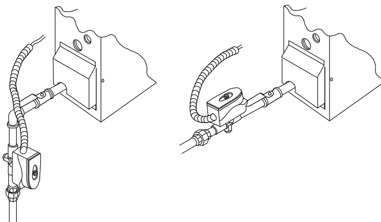
DIAGRAM 4: TYPICAL DRAIN INSTALLATIONS
